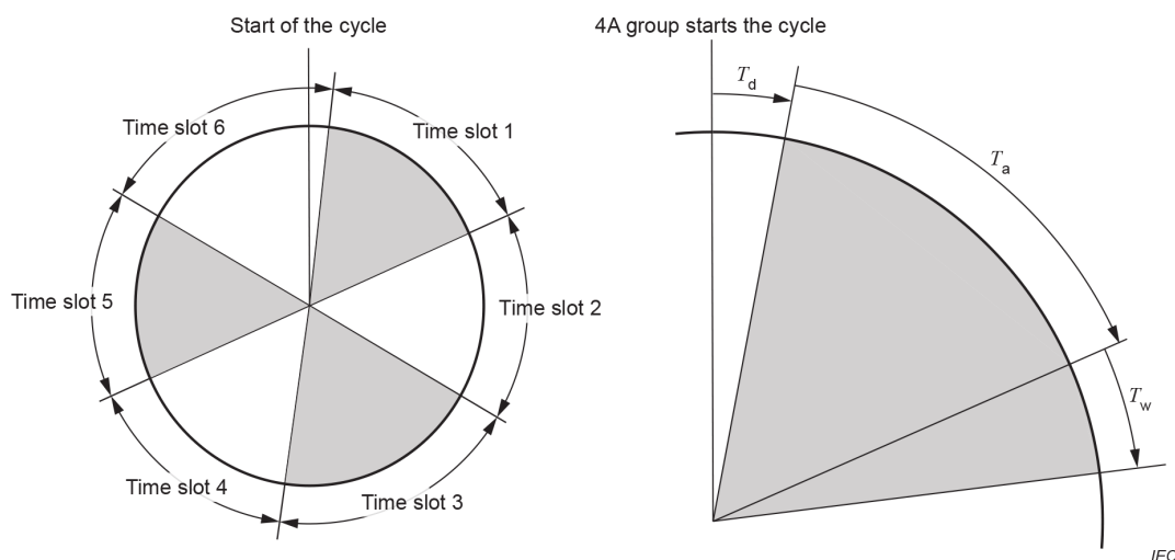
Figure F.1 – "Spinning wheel" mode – one minute transmission cycle that starts with a 4A group
